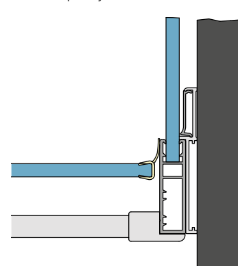
Detail A – pôdorys
