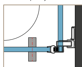
Detail A - pôdorys
